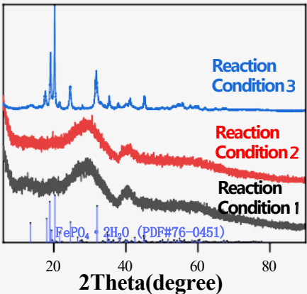
Mastery of the phase transition behaviour of iron phosphate: the monoclinic crystal structure is more stable, contributing to improved product consistency.
